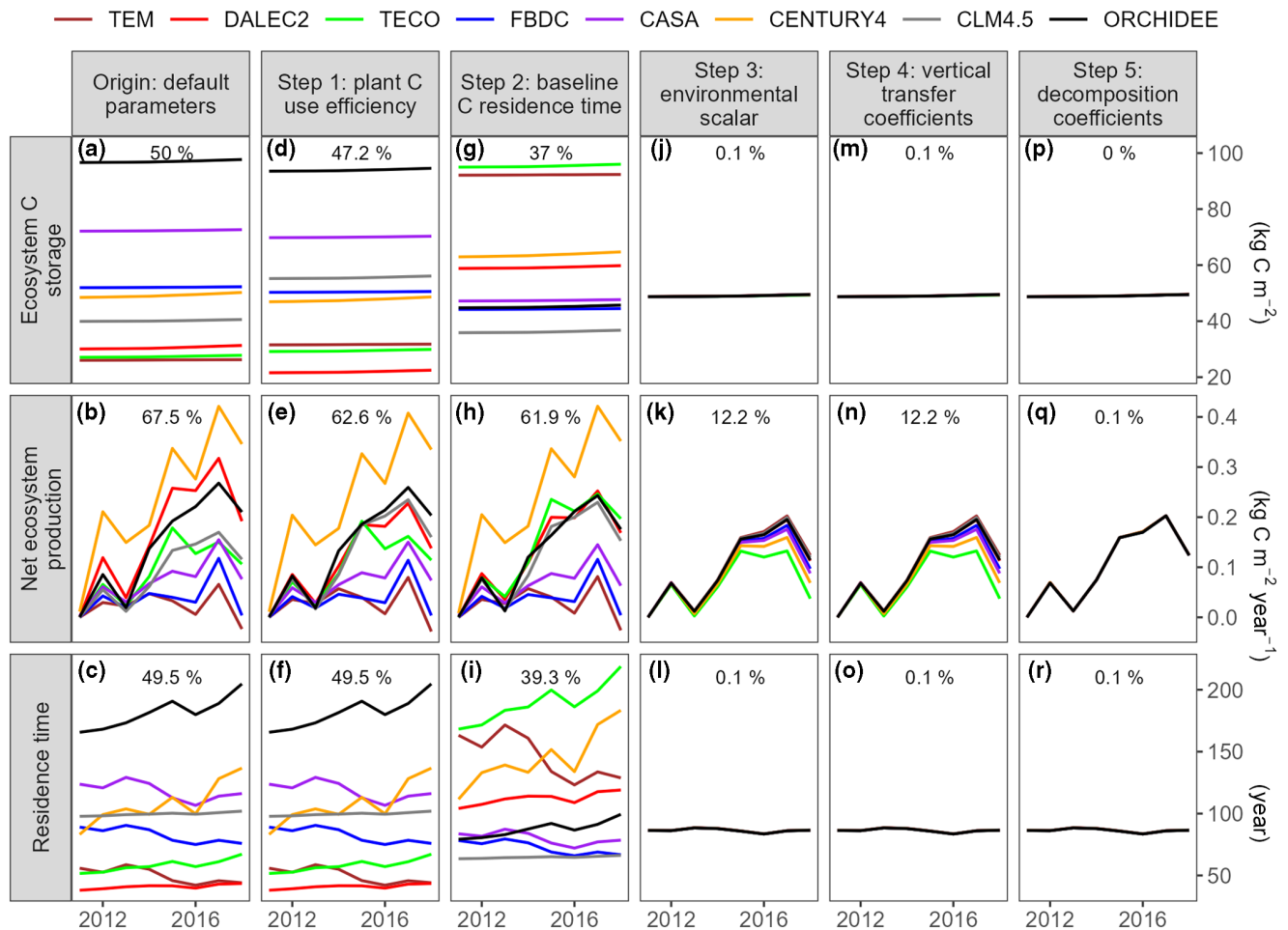
FIGURE 5 Across-model spread in ecosystem C dynamics are shrinkage after standardizing parameter values. Simulated ecosystem C storage, net ecosystem production, and C residence time in the (a–c) original model run and (d–r) model runs after Steps 1–5, respectively. Origin model run indicates model simulations with the default parameter values. Steps 1–5 indicate model simulations after sequentially standardizing plant C use efficiency, baseline C residence time, environmental scalar, and vertical transfer coefficients, and homogenizing decomposition coefficients. Percentage in each subpanel indicates the coefficient of variance of time-averaged simulations. [Colour figure can be viewed at wileyonlinelibrary.com ]
