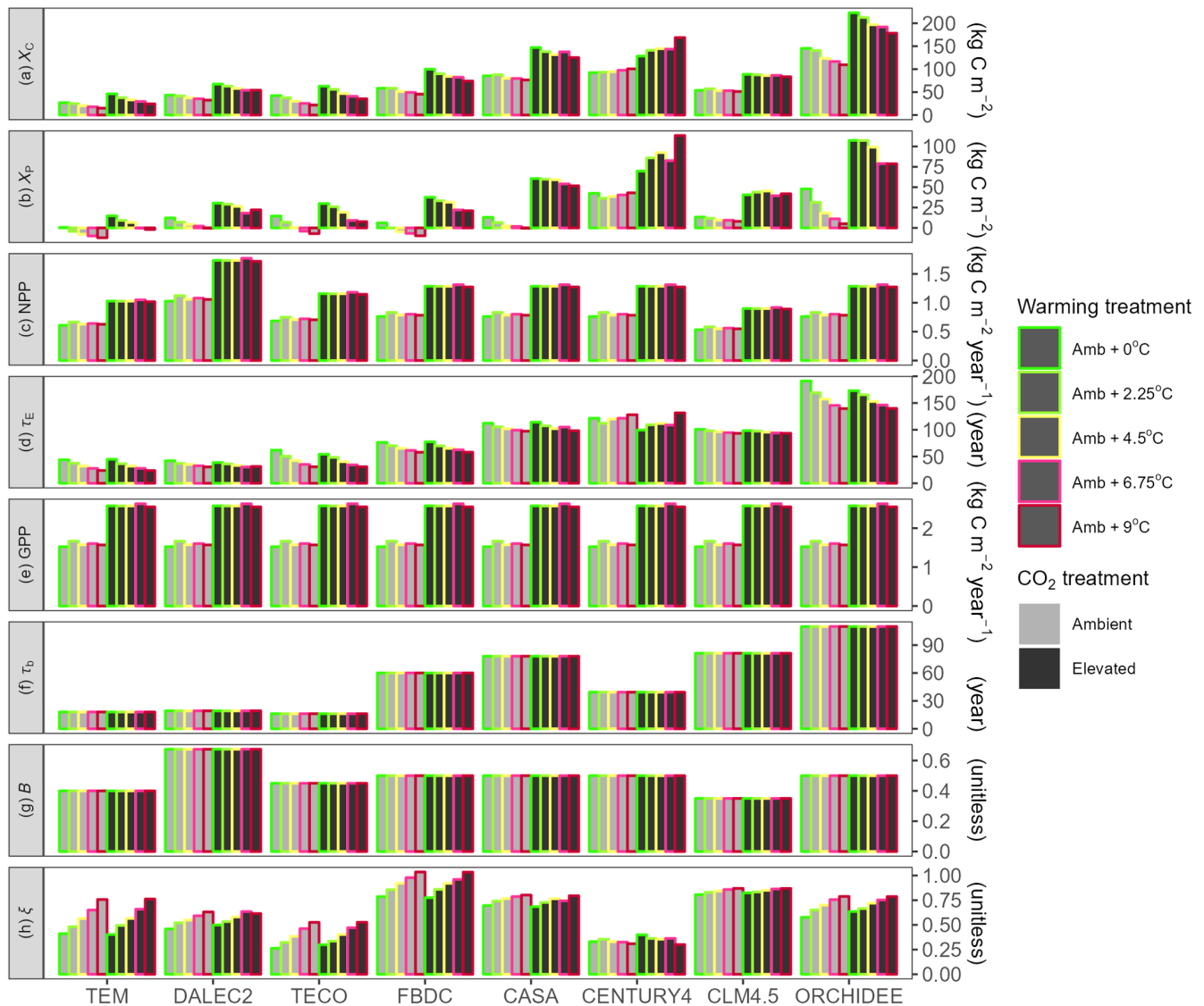
FIGURE 8 Traceable model components under different experimental treatments. Comparisons of (a) C storage capacity ( X_c ), (b) C storage potential ( X_p ), (c) net primary production (NPP), (d) ecosystem C residence time ( \tau_E ), (e) gross primary production (GPP), (f) baseline C residence time ( \tau_0 ), (g) C allocation coefficients ( B ), and (h) environmental scalar ( \xi ) among models in a factorial combination of five warming levels (ambient condition +0, 2.25, 4.5, 6.75, and 9.0°C, respectively) and two CO 2 concentration levels (ambient CO 2 , and elevated CO 2 up to 900ppm, respectively). [Colour figure can be viewed at wileyonlinelibrary.com ]
