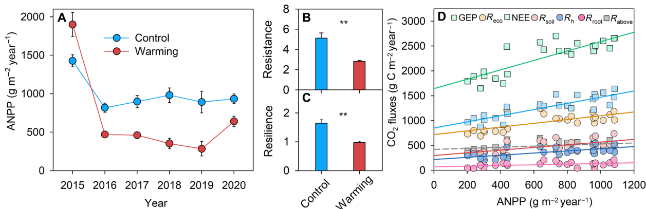
Fig. 3. Warming effect on ecosystem resistance and resilience. Warming effects on ANPP ( \text{g dry matter m}^{-2} \text{ year}^{-1} ) (A) and its resistance (B) and resilience (C) to flooding. Error bars represent SE across replicates ( n = 4 ). **P < 0.01 . (D) The relationship between carbon fluxes and ANPP across all plots and years. The solid line represents a statistically significant correlation ( P < 0.05 ) of ANPP with gross ecosystem productivity (GEP; \text{g C m}^{-2} \text{ year}^{-1} ), ecosystem respiration ( R_{\text{eco}} ; \text{g C m}^{-2} \text{ year}^{-1} ), net ecosystem \text{CO}_2 exchange (NEE; \text{g C m}^{-2} \text{ year}^{-1} ), soil respiration ( R_{\text{soil}} ; \text{g C m}^{-2} \text{ year}^{-1} ), soil heterotrophic respiration ( R_{\text{h}} ; \text{g C m}^{-2} \text{ year}^{-1} ), and root respiration ( R_{\text{root}} ; \text{g C m}^{-2} \text{ year}^{-1} ). The squares represent \text{CO}_2 uptake. The circles represent \text{CO}_2 or \text{CH}_4 release. The dashed line shows the insignificant relationship between aboveground respiration ( R_{\text{above}} ; \text{g C m}^{-2} \text{ year}^{-1} ) and ANPP ( P > 0.05 ).
