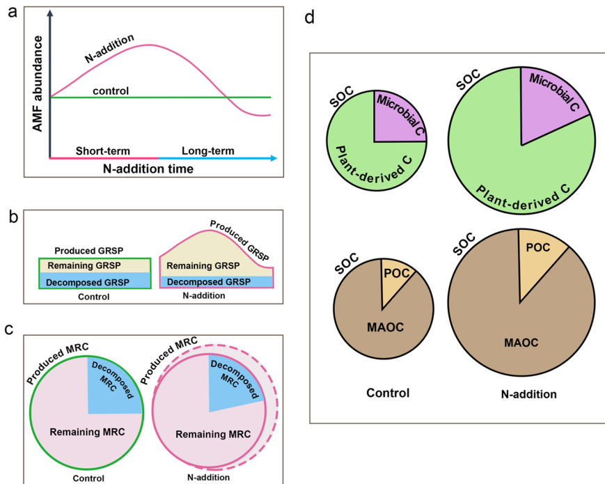
Fig. 6 Conceptual diagrams showing how the accumulation of glomalin-related soil protein (GRSP) and microbial residual C (MRC) contribute to the soil organic carbon (SOC) contents under N addition, and the underlying microbial mechanisms. (a) The abundance of arbuscular mycorrhizal fungi (AMF) initially increases with the alleviation of N-limitation and then declines over time as soils become N-saturated. (b) Conceptual diagram illustrating how the production and decomposition of GRSP remains constant in the controls, whereas the production of GRSP is initially stimulated by N-addition and the decomposition of GRSP is suppressed, resulting in greater overall accumulation of GRSP with N-addition. (c)
