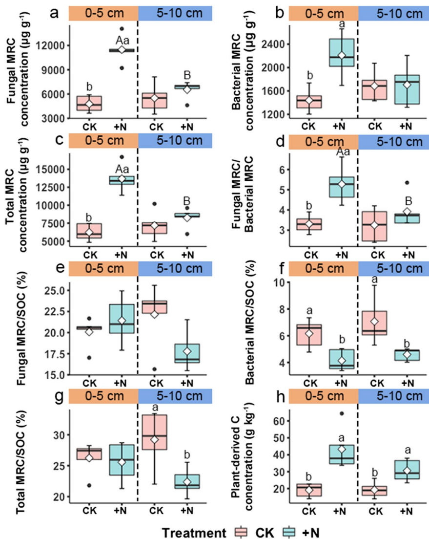
Fig. 3 Microbial residual carbon (MRC) in soils and its contribution to soil organic carbon (SOC), showing the concentrations of (a) fungal MRC, (b) bacterial MRC, (c) total MRC, and (d) the ratio of fungal to bacterial MRC; and the contributions of (e) fungal MRC, (f) bacterial MRC, (g) total MRC to SOC, and (h) plant-input C concentration, where CK is control and +N is N addition; capital letters denote significant differences between soil depths under the same addition treatment and lowercase letters denote significant differences between addition treatments at the same soil depth at P < 0.05 . Boxes denote the 25 th and 75 th percentiles and median lines are given for n = 5 plots per treatment and depth, diamonds represent mean values, whiskers indicate values up to 1.5 \times the interquartile range, and dots indicate outliers
