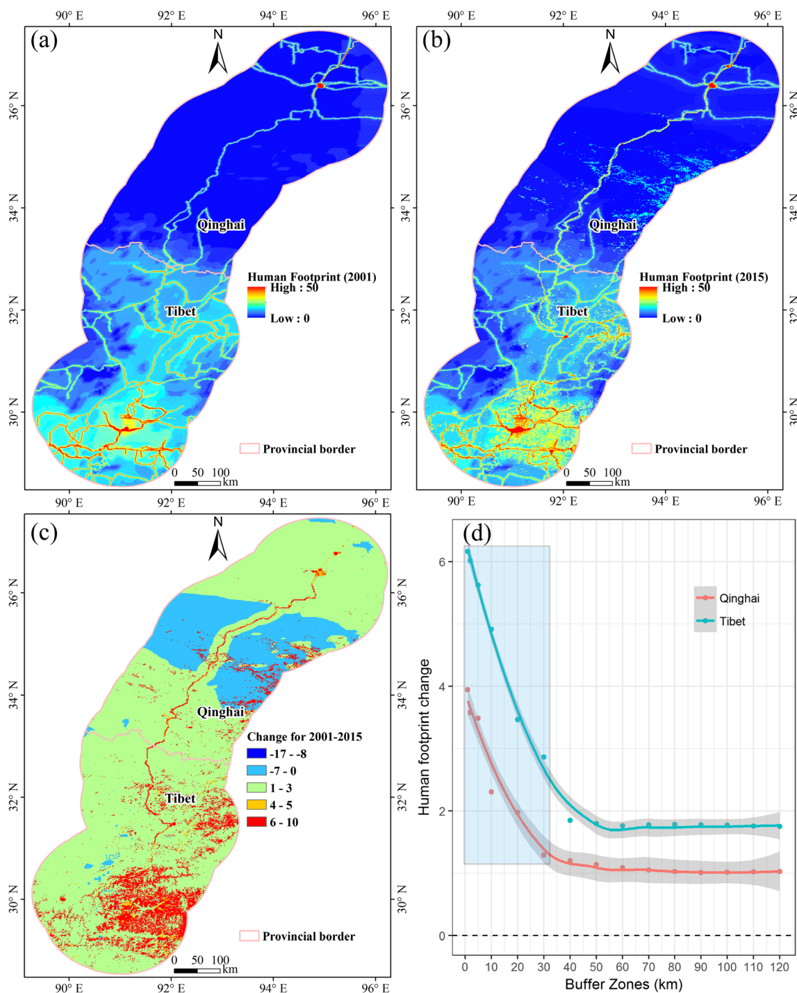
Fig. 3 Change in the human footprint in the Qinghai-Tibet Engineering Corridor (QTEC). a Human footprint map for 2001. b Human footprint map for 2015. c Change in human pressure for 2001–2015. d Change in
