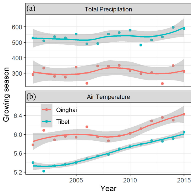
Fig. 2 Growing season meteorological factors for the 120-km buffer zone in the Qinghai and Tibet regions of the Qinghai-Tibet Engineering Corridor (QTEC) from 2001 to 2015. a Total precipitation (mm). b Mean air temperature (°C). The grey-shaded area depicts 95% confidence intervals
