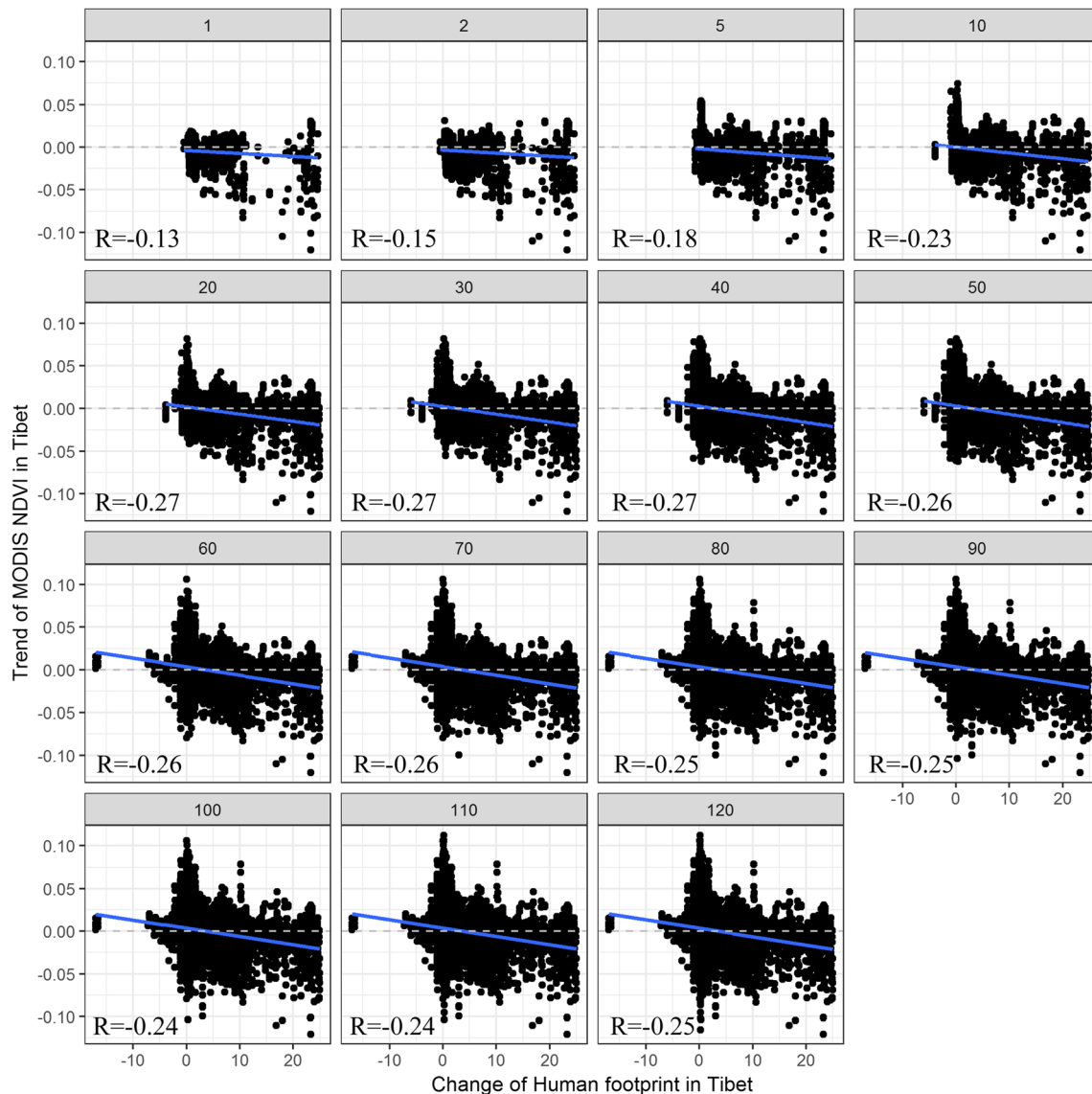
Fig. 7 Spatial relationship between the growing season MODIS normalized difference vegetation index (NDVI) trend and changes in the human footprint for 1- to 120-km buffer zones in Tibet. The number
