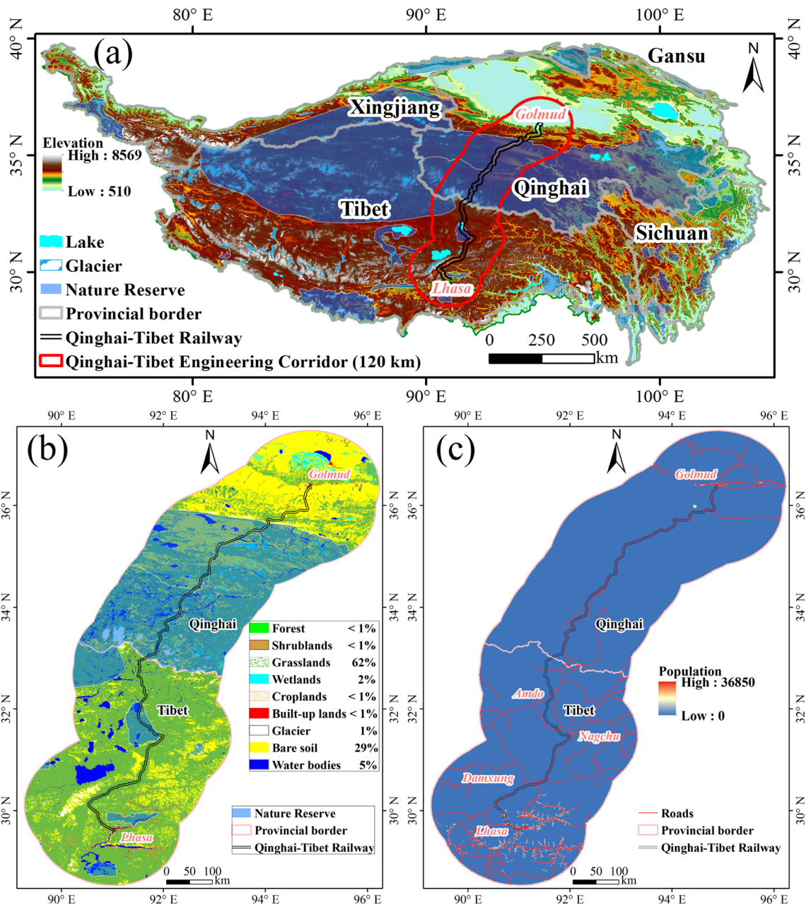
Fig. 1 Maps showing the location of the study area. a The Qinghai-Tibet Plateau (QTP) and Qinghai-Tibet Engineering Corridor (QTEC). The red border is the 120-km buffer zone of the railway. b Distribution of
