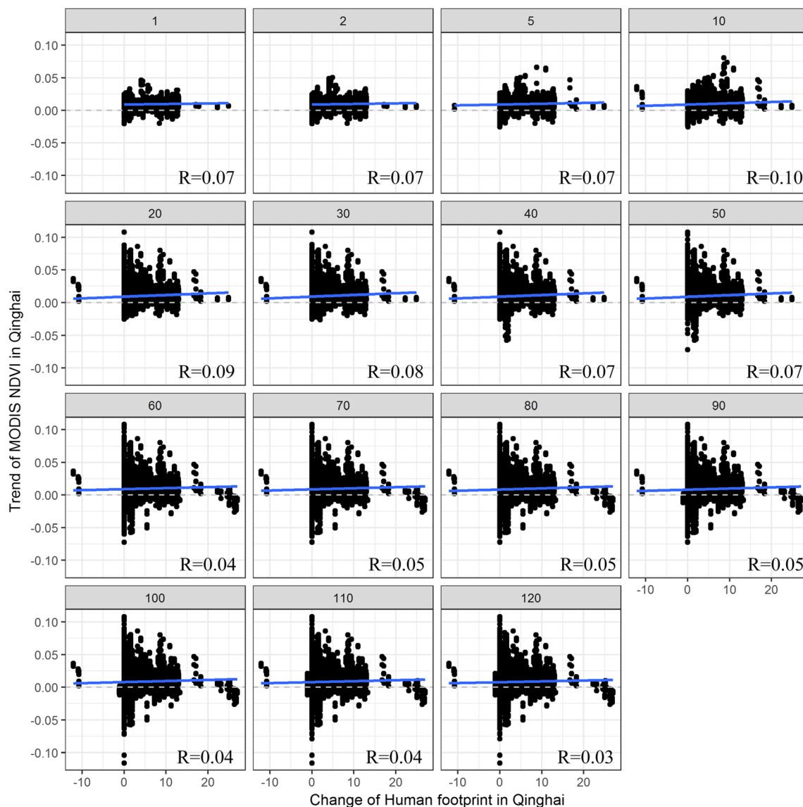
Fig. 6 Spatial relationship between the growing season MODIS normalized difference vegetation index (NDVI) trend and changes in the human footprint for 1- to 120-km buffer zones in Qinghai. The
