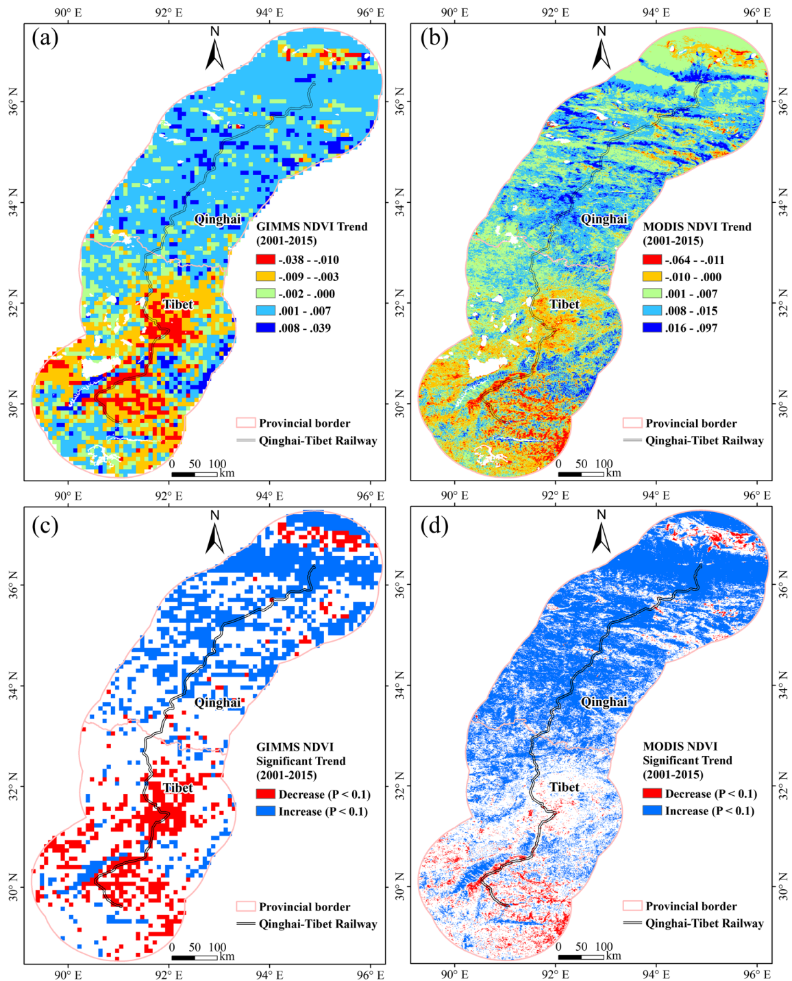
Fig. 4 Growing season normalized difference vegetation index (NDVI) change trends and significance levels from 2001 to 2015. a GIMMS NDVI change trend obtained with the linear regression method. b MODIS NDVI change trend obtained with the linear regression method.
