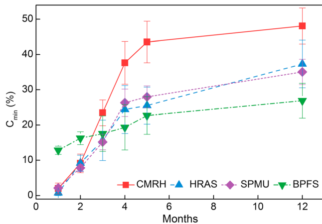
Figure 7. The percentage of compost carbon mineralized ( C_{\min} , %) over different months of decomposition. Vertical bars denote standard errors ( n = 4 ).
