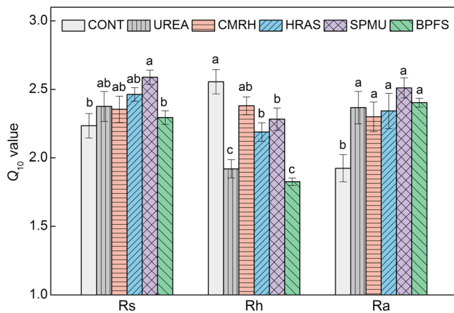
Figure 5. The Q_{10} values of total soil respiration (Rs), heterotrophic (Rh), and autotrophic respiration (Ra) in different fertilization treatments. Vertical bars denote standard errors ( n = 4 ). Different letters indicate significant differences at P < 0.05 .
