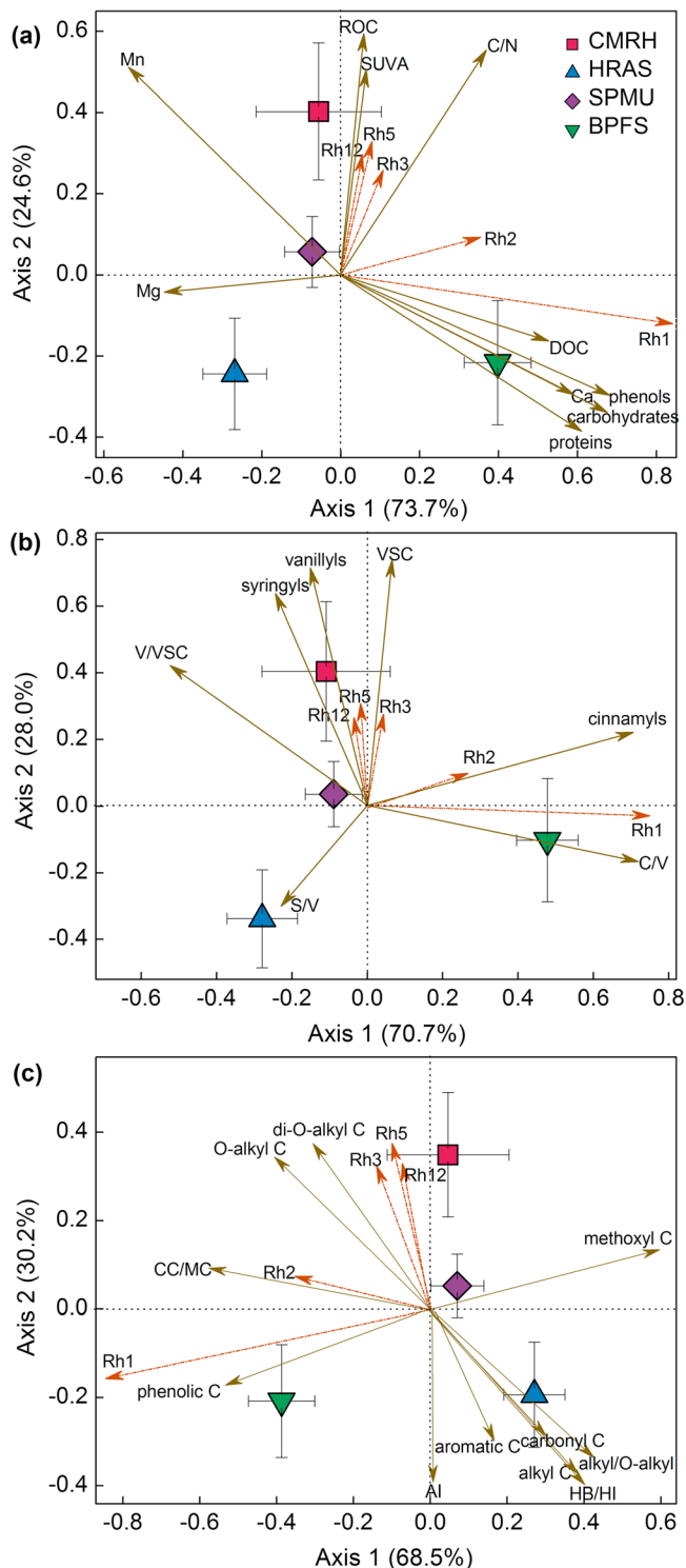
Figure 4. Redundancy analysis (RDA) diagrams showing the relationships between cumulative heterotrophic respiration (Rh) during the period from 0 to 1, 2, 3, 5, and 12 months in the compost treatments and general properties of compost composition and metal contents (a), lignin parameters (b), and characteristics determined by NMR (c).
