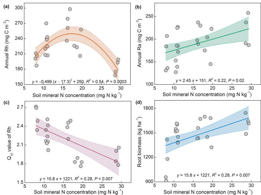
Figure 3. Relationships between annual heterotrophic respiration ( R_h ; a), autotrophic respiration ( R_a ; b), Q_{10} values of R_h (c), and root biomass (d) with annual mean soil mineral nitrogen concentration. Shaded areas indicate the 95% confidence intervals.
