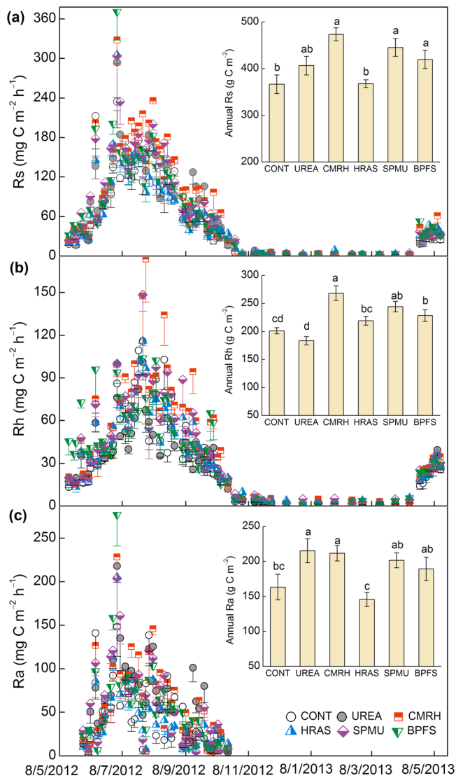
Figure 2. Seasonal dynamics and annual emission of soil respiration (Rs, a), heterotrophic (Rh, b), and autotrophic respiration (Ra, c) in different fertilization treatments. Vertical bars denote standard errors ( n = 4 ). Different letters indicate significant differences at P < 0.05 .
