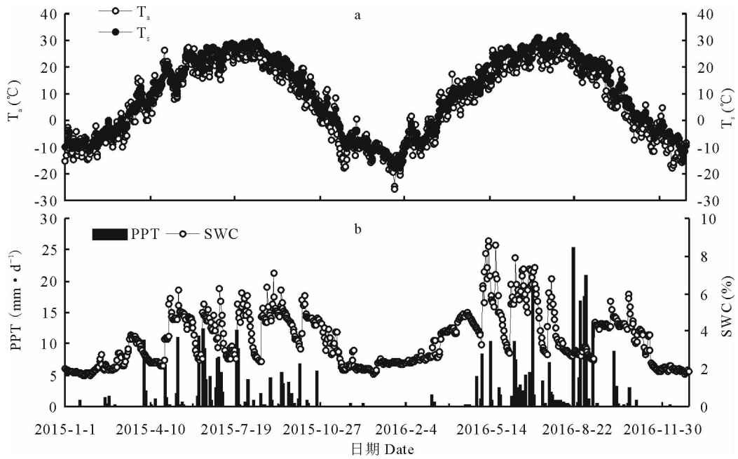
图 1 空气温度( T_a )、5 cm 土壤温度( T_s )、5 cm 土壤体积含水量(SWC)和日降水量(PPT)的季节变化 Fig. 1 Seasonal variation of air temperature ( T_a ), soil temperature at 5 cm depth ( T_s ), soil water content at 5 cm depth (SWC) and precipitation (PPT) in sandy grassland ecosystem
