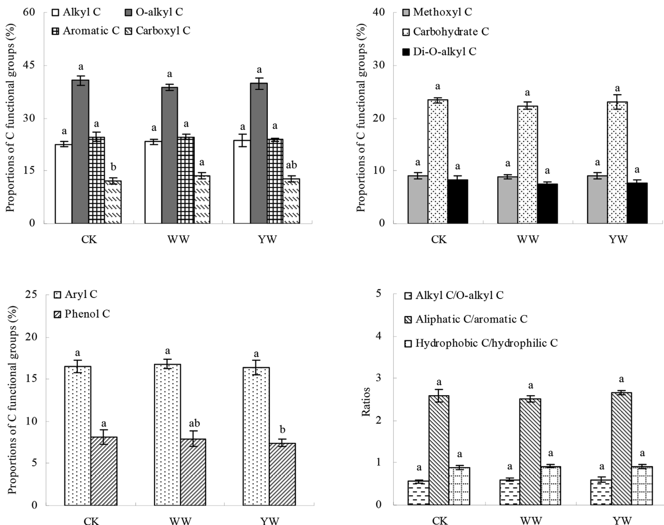
Fig. 6. Distribution of different carbon (C) functional groups in bulk soil samples obtained from solid-state ^{13}\text{C} CPMAS NMR spectra under different treatments. Vertical bars represent standard deviation of the mean ( n = 5 ). Different letters indicate significant differences among treatments ( p < 0.05 ). CK: unwarmed control; WW: winter warming; YW: year-round warming. Aliphatic C/aromatic C = (alkyl C + O-alkyl C)/aromatic C; Hydrophobic C/hydrophilic C = (alkyl C + aromatic C)/(O-alkyl C + carboxyl C).
