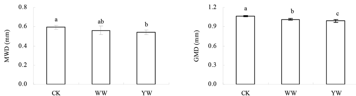
Fig. 9. Mean weight diameter (MWD) and geometric mean diameter (GMD) of water-stable aggregates in soil under different treatments. Vertical bars represent standard deviation of the mean ( n = 5 ). Different letters indicate significant differences among treatments ( p < 0.05 ). CK: unwarmed control; WW: winter warming; YW: year-round warming.
