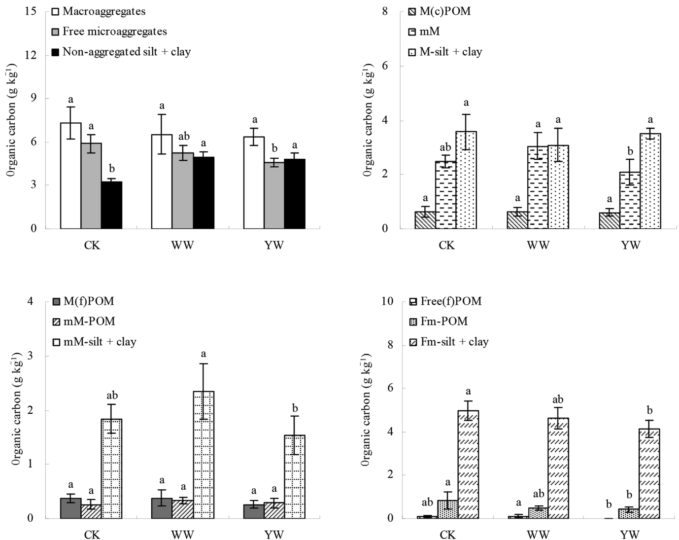
Fig. 7. Organic carbon contents of hierarchical aggregates in soil under different treatments. Vertical bars represent standard deviation of the mean ( n = 5 ). Different letters indicate significant differences among treatments ( p < 0.05 ). CK: unwarmed control; WW: winter warming; YW: year-round warming. For other abbreviations, see Fig. 2.
