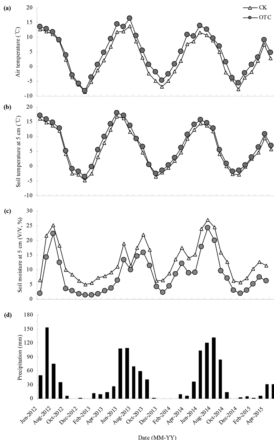
Fig. 3. Average air temperature (a), soil temperature (b), soil moisture at 5 cm depth (c) and precipitation (d) in the open top chambers (OTCs) and control (CK) during the experiment period from June 2012 to May 2015.
