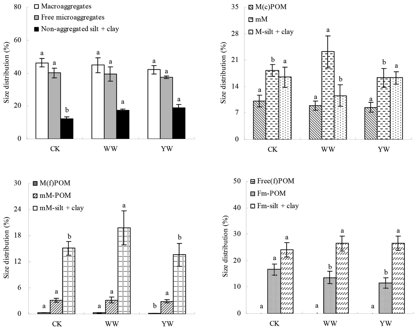
Fig. 8. Size distribution of hierarchical aggregates in soil under different treatments. Vertical bars represent standard deviation of the mean ( n = 5 ). Different letters indicate significant differences among treatments ( p < 0.05 ). CK: unwarmed control; WW: winter warming; YW: year-round warming. For other abbreviations, see Fig. 2.
