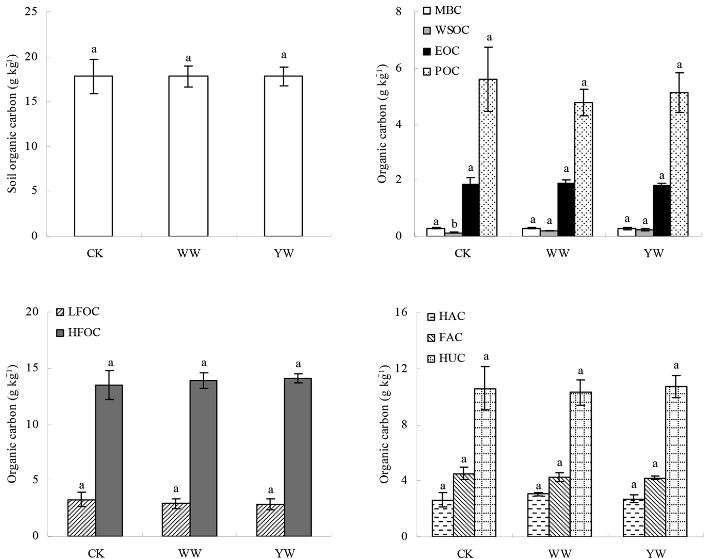
Fig. 4. Contents of soil organic carbon and its fractions under different treatments. Vertical bars represent standard deviation of the mean ( n = 5 ). Different letters indicate significant differences among treatments ( p < 0.05 ). CK: unwarmed control; WW: winter warming; YW: year-round warming. WSOC: water-soluble organic carbon; MBC: microbial biomass carbon; EOC: easily oxidizable organic carbon; POC: particulate organic carbon; LFOC: light fraction organic carbon; HFOC: heavy fraction organic carbon; HAC: humic acid carbon; FAC: fulvic acid carbon; HUC: humin carbon.
