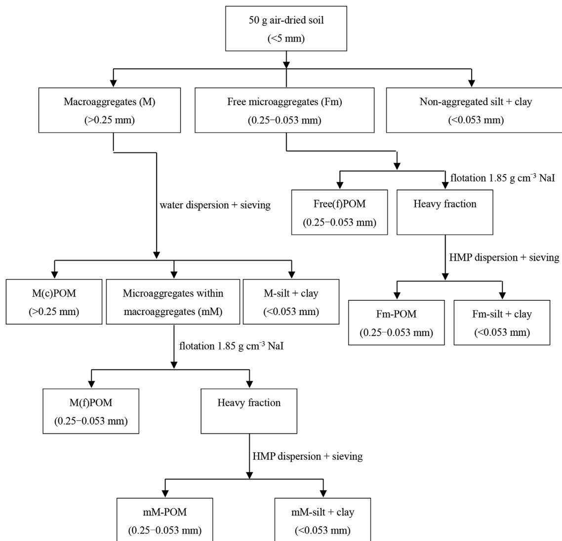
Fig. 2. Fractionation scheme to isolate soil aggregates fractions. M(c)POM: coarse particulate organic matter (POM) inside macroaggregates but outside microaggregates; M(f)POM: non-occluded fine POM inside macroaggregates but outside microaggregate; mM-POM: POM inside microaggregates-within-macroaggregates; M-silt + clay: silt- and clay-sized fractions inside macroaggregates; mM-silt + clay: silt- and clay-sized fractions inside microaggregates-within-macroaggregates; Free (f)POM: non-occluded fine POM not inside any aggregates; Fm-POM: POM inside free microaggregates; Fm-silt + clay: silt- and clay-sized fractions inside free microaggregates (adapted from Yan et al., 2012; and O'Brien and Jastrow, 2013). HMP: sodium hexametaphosphate.
