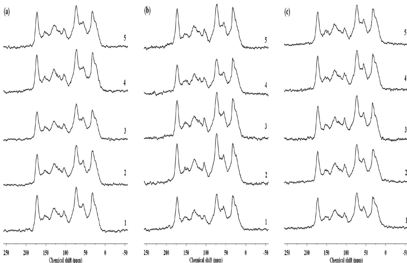
Fig. 5. Solid-state ^{13}\text{C} CPMAS NMR spectra of bulk soil samples under unwarmed control (CK) (a), winter warming (WW) (b) and year-round warming (YW) (c). The graphs listed 1 to 5 in each subplot represent the five replicates from each treatment.
