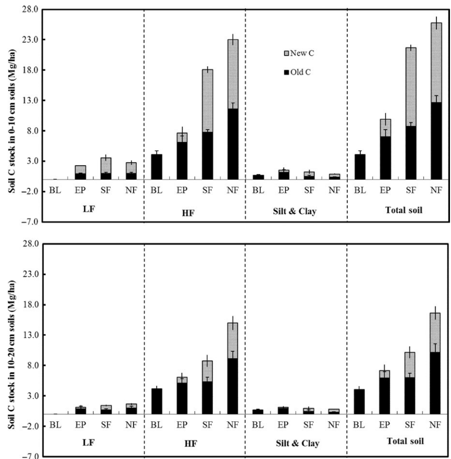
FIGURE 7 Stocks of new and old carbon in different soil density fractions, soil aggregates and the bulk soil at different soil depths in four land-use types after the restoration of degraded land in tropical South China, where BL is bare land, EP is Eucalyptus plantation, SF is secondary forest, and NF is natural old-growth forest, LF is the light density fraction, HF is the heavy fraction, error bars indicate standard errors for n = 4
