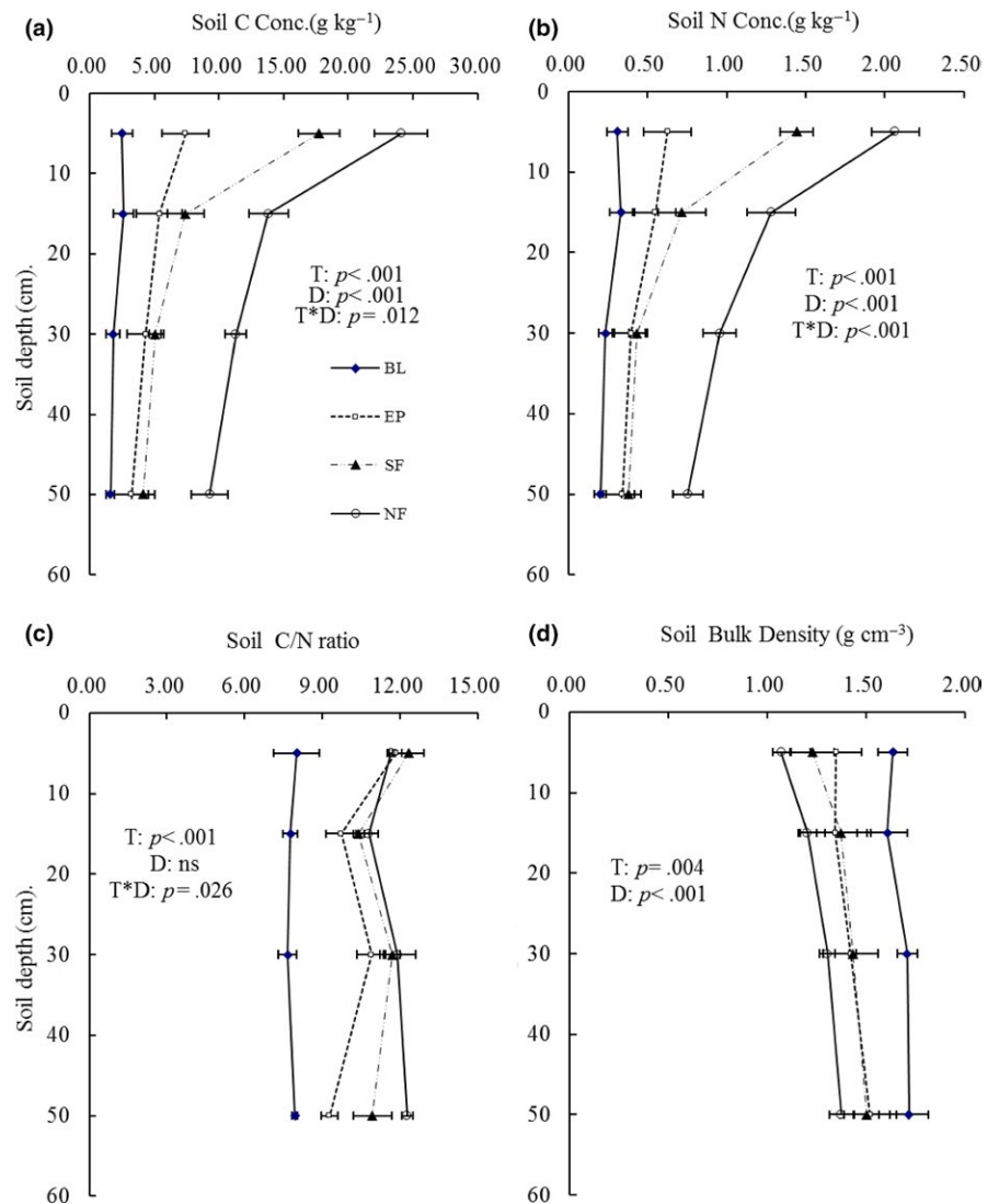
FIGURE 4 Depth distribution of (a) soil C, (b) soil N, (c) soil C/N ratio and (d) bulk density in four land-use types after the restoration of degraded land in tropical South China, where BL is bare land, EP is Eucalyptus plantation, SF is secondary forest, and NF is natural old-growth forest; significance values are given for main effects from a linear mixed model (see statistical analysis), where T is the effect of land-use type and D is the effect of soil depth; error bars indicate standard errors for n = 4
