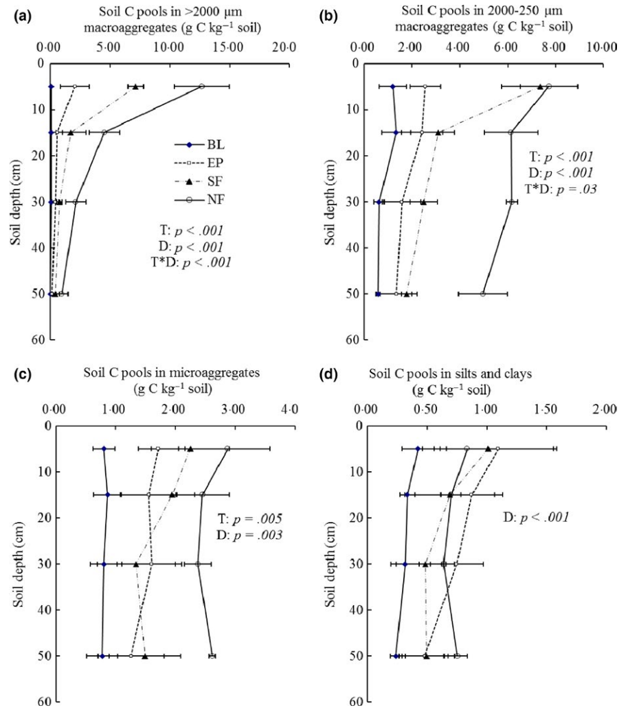
FIGURE 6 Soil aggregate size fractions (a, >2000\ \mu\text{m} ; b, 2000\text{--}250\ \mu\text{m} ; c, microaggregate; d, silts and clays) at different soil depths in four land-use types after the restoration of degraded land in tropical South China, where BL is bare land, EP is Eucalyptus plantation, SF is secondary forest, and NF is natural old-growth forest; significance values are given for main effects from a linear mixed model, where T is the effect of land-use type and D is the effect of soil depth; error bars indicate standard errors for n = 4
