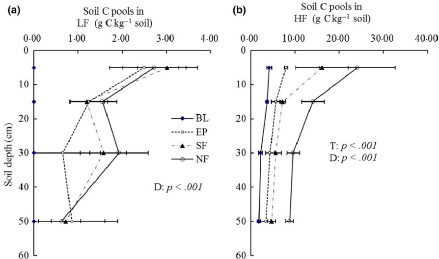
FIGURE 5 Soil carbon pools in the light density fraction (LF, a) and heavy density fraction (HF, b) at different soil depths in four land-use types after the restoration of degraded land in tropical South China, where BL is bare land, EP is Eucalyptus plantation, SF is secondary forest, and NF is natural old-growth forest; significance values are given for main effects from a linear mixed model, where T is the effect of land-use type and D is the effect of soil depth; error bars indicate standard errors for n = 4
