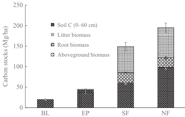
FIGURE 3 Total carbon stocks and carbon pools in four land-use types after the restoration of degraded land in tropical South China, where BL is bare land, EP is Eucalyptus plantation, SF is secondary forest, and NF is natural old-growth forest; error bars indicate standard errors for n = 4 per carbon pool
