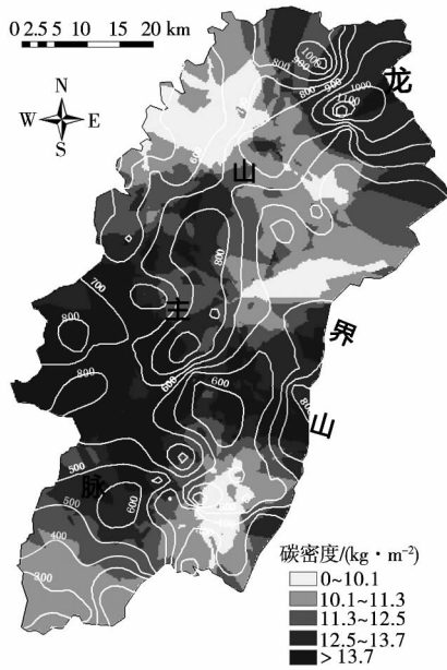
图1 龙山县0~100 cm土层土壤有机碳密度地形空间分布图 Fig. 1 The distribution map of soil organic carbon density of 0~100 cm soil profile based on topography in Longshan county
