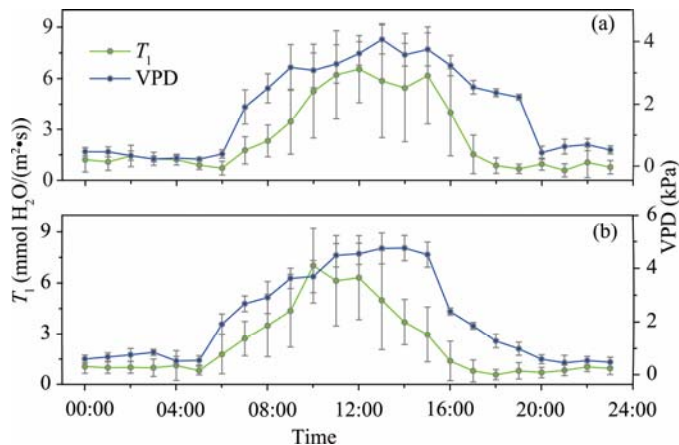
Fig. 2 Averaged diurnal course of transpiration T_1 and leaf-to-air vapor pressure deficit (VPD) at leaf level on Julian days of 188–189 (a) and 218–219 (b). Error bars represent the standard deviation of replicate measurements on different leaves.
