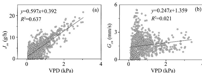
Fig. 7 Nighttime half-hourly whole plant transpiration rate ( J_{sn} ; a) and canopy bulk stomatal conductance ( G_{cn} ; b) of maize in response to air VPD
